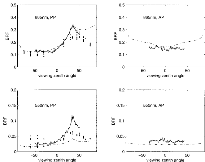
Fig. 10. Comparison of the modeled (dash-dot line) (using the model without the multiscale hotspot function) bidirectional reflectance factor (BRF) in the principal plane (left) and across the principal plane (right) in the red (550 nm) (bottom) and near infrared (865 nm) (top) with POLDER measurement (solid line) and PARABOLA measurements (dots) in the old black spruce forest in the southern site (SOBS) of BOREAS in 1994. The solar zenith angle is 36^\circ .
