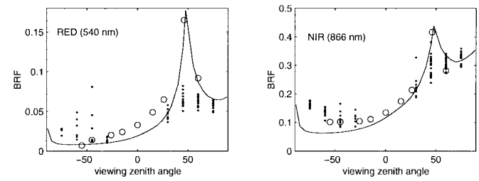
Fig. 9. Comparison of the modeled (solid line) bidirectional reflectance factor (BRF) in the principal plane in the red spectral range (540 nm) (left) and near-infrared (866 nm) with ASAS (circles) and PARABOLA measurements (dots) in the old black spruce forest in the southern site (SOBS) of BOREAS in 1994. The solar zenith angle is 47.7^\circ .
