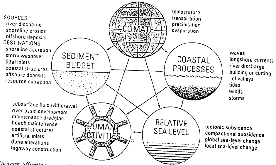
Factors affecting coastal environments are interwoven in an intricate web. (Modified from Pilkey and others, 1989, Coastal land loss; 28th International Geological Congress Short Course: Washington, D.C., American Geophysical Union, 73 p.)
